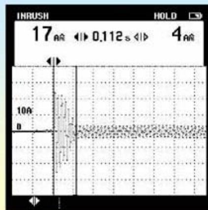
Figure 7N Example of switch-on inrush current (captured with a Fluke 43B and current probe)
